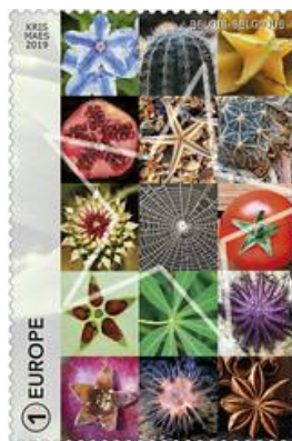
4862 (1)E Collection of star shapes in nature
